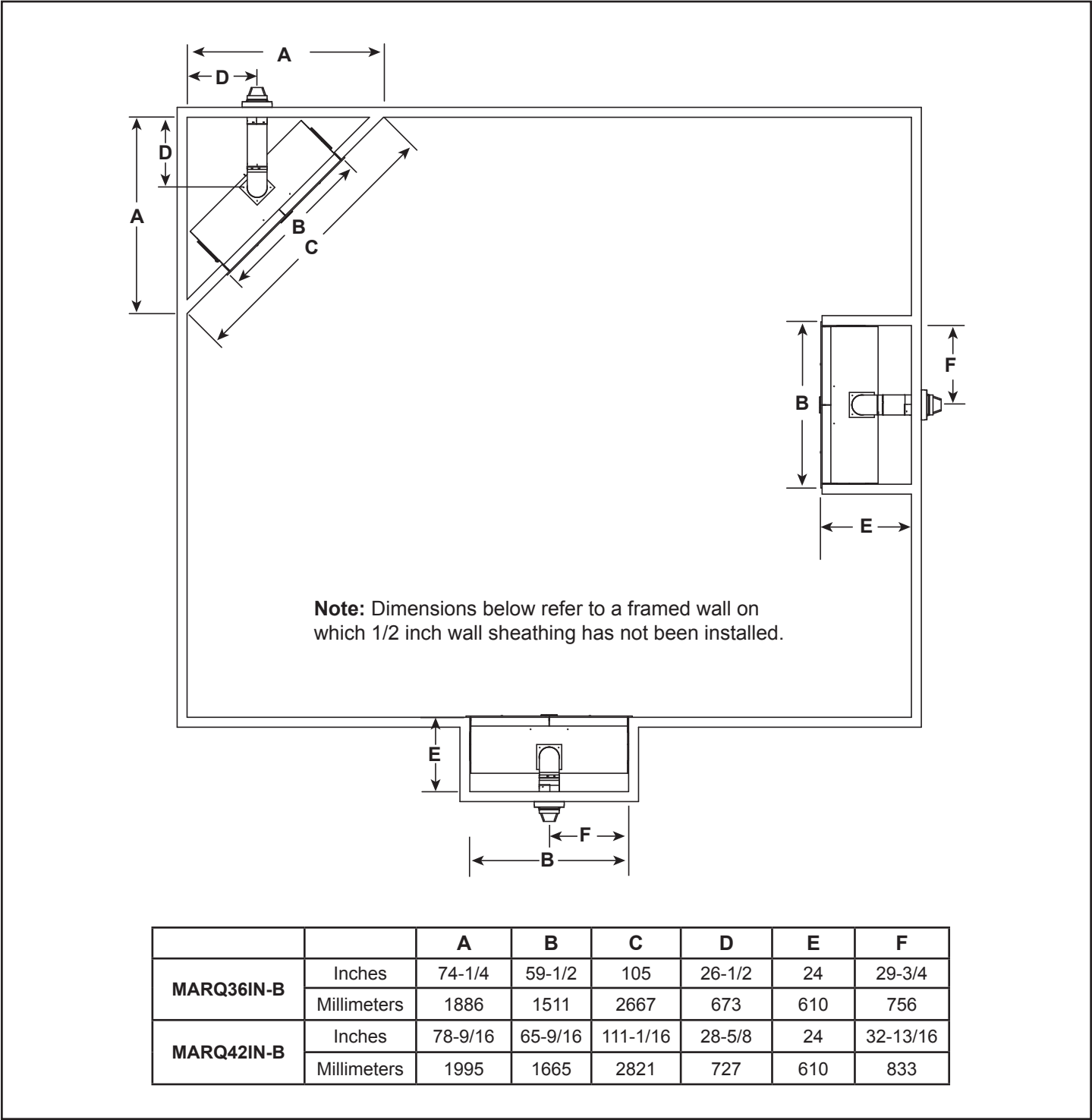
Figure 3.4 Appliance Locations
