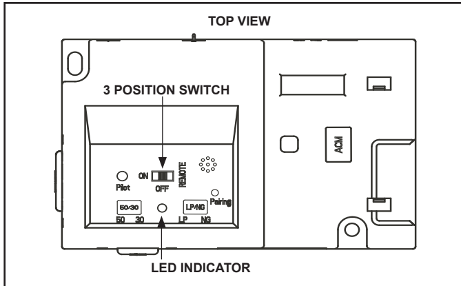
Figure 11.5 IFT-ECM
