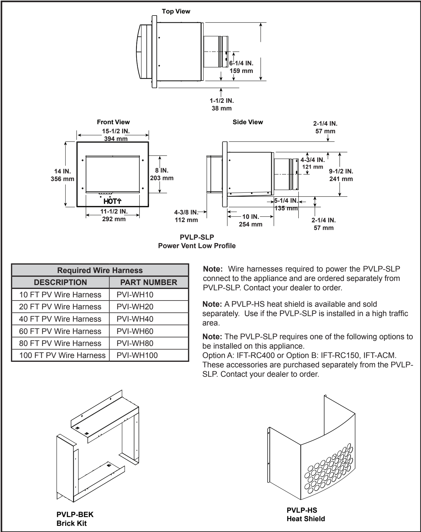
Figure 12.5 PVLP-SLP Vent Components
