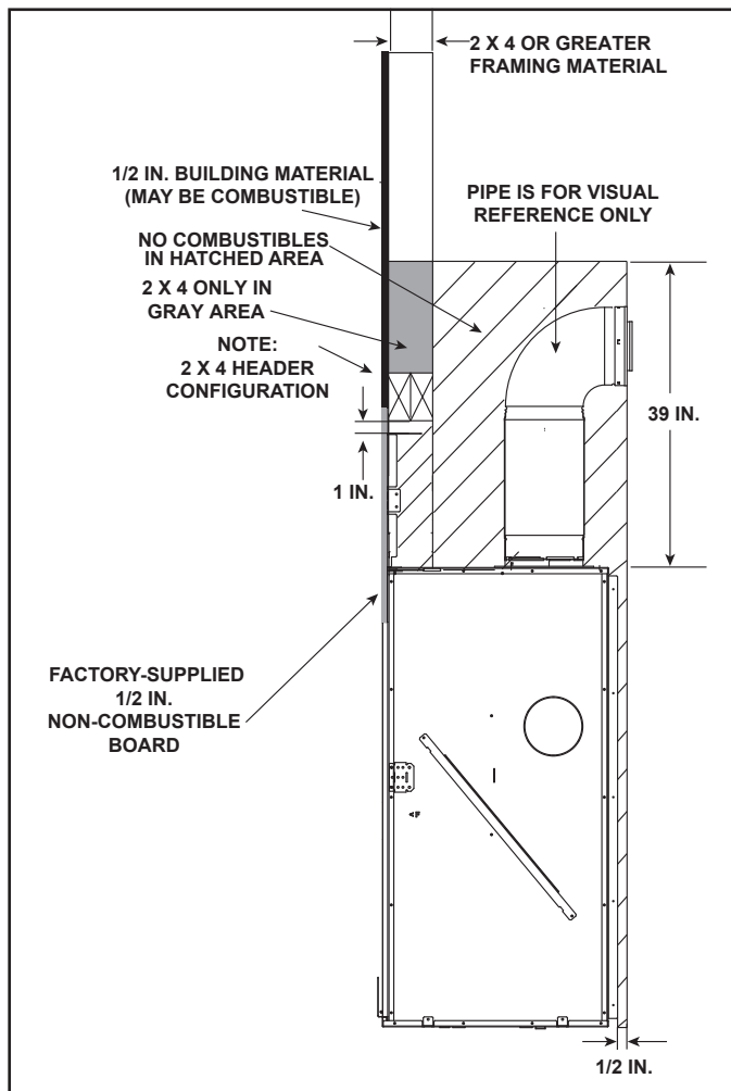
Figure 10.8 Non-Combustible Zone
