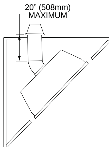
RIGID VENTING
