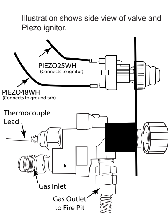
Fig. 6 TMSI typical installation.
