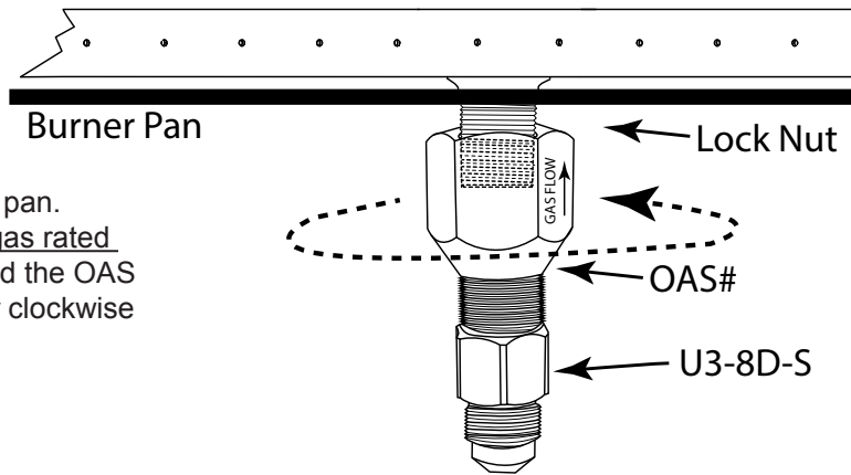
Fig. 5 Installing OAS (orifice) to burner tube.
