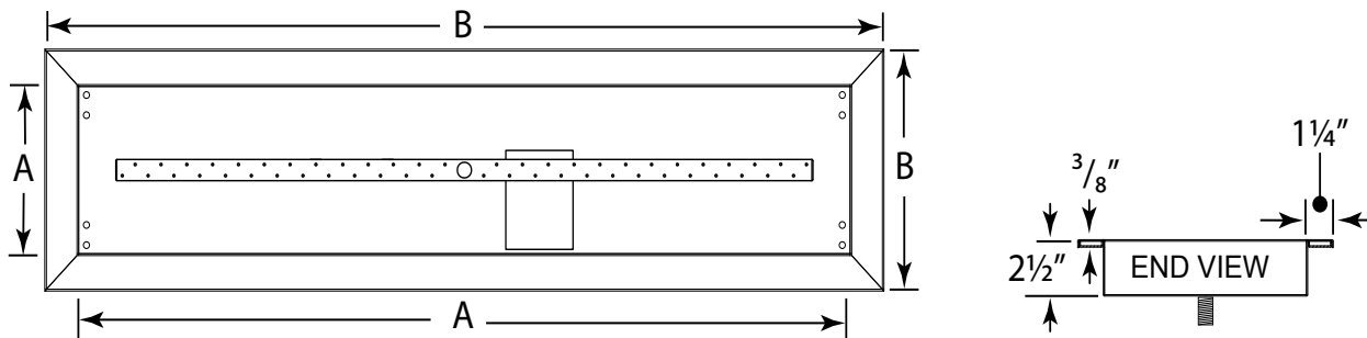
Fig. 3 T-style burner pan specifications.
