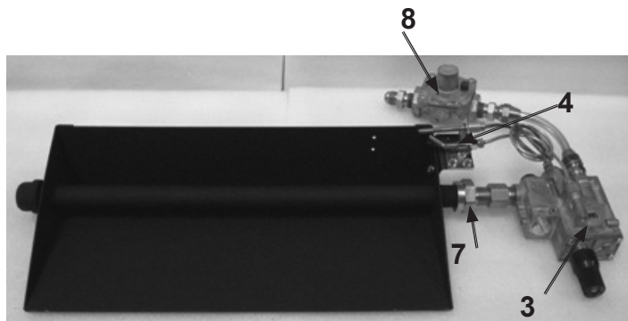
Hearth Kit Assemblies- LP
